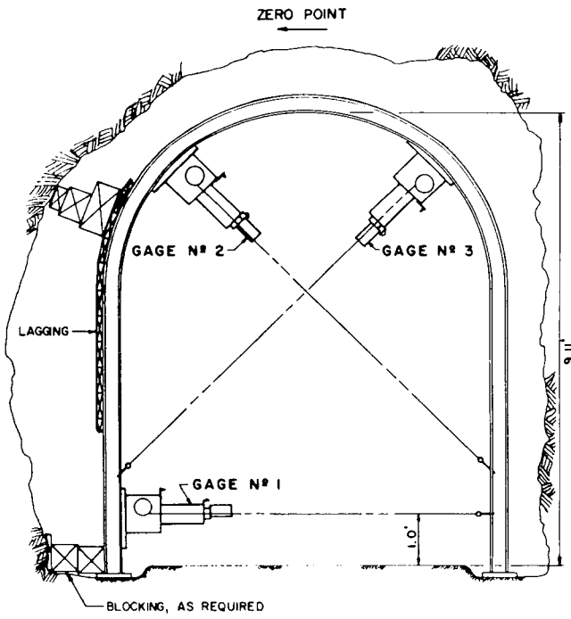
Fig. 3—Gauge setup in station 2+85, drift U12e.05, Logan event.
